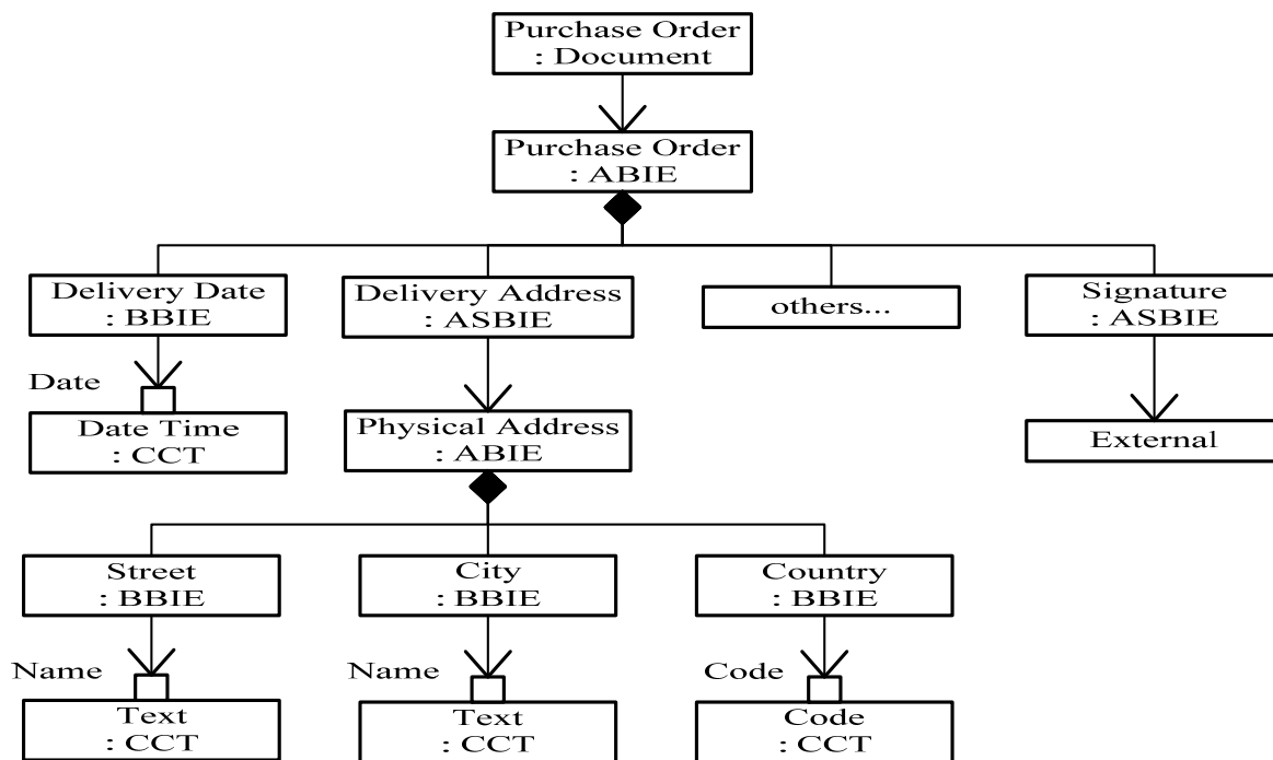
Figure 3: Sample information model for purchase order documents
