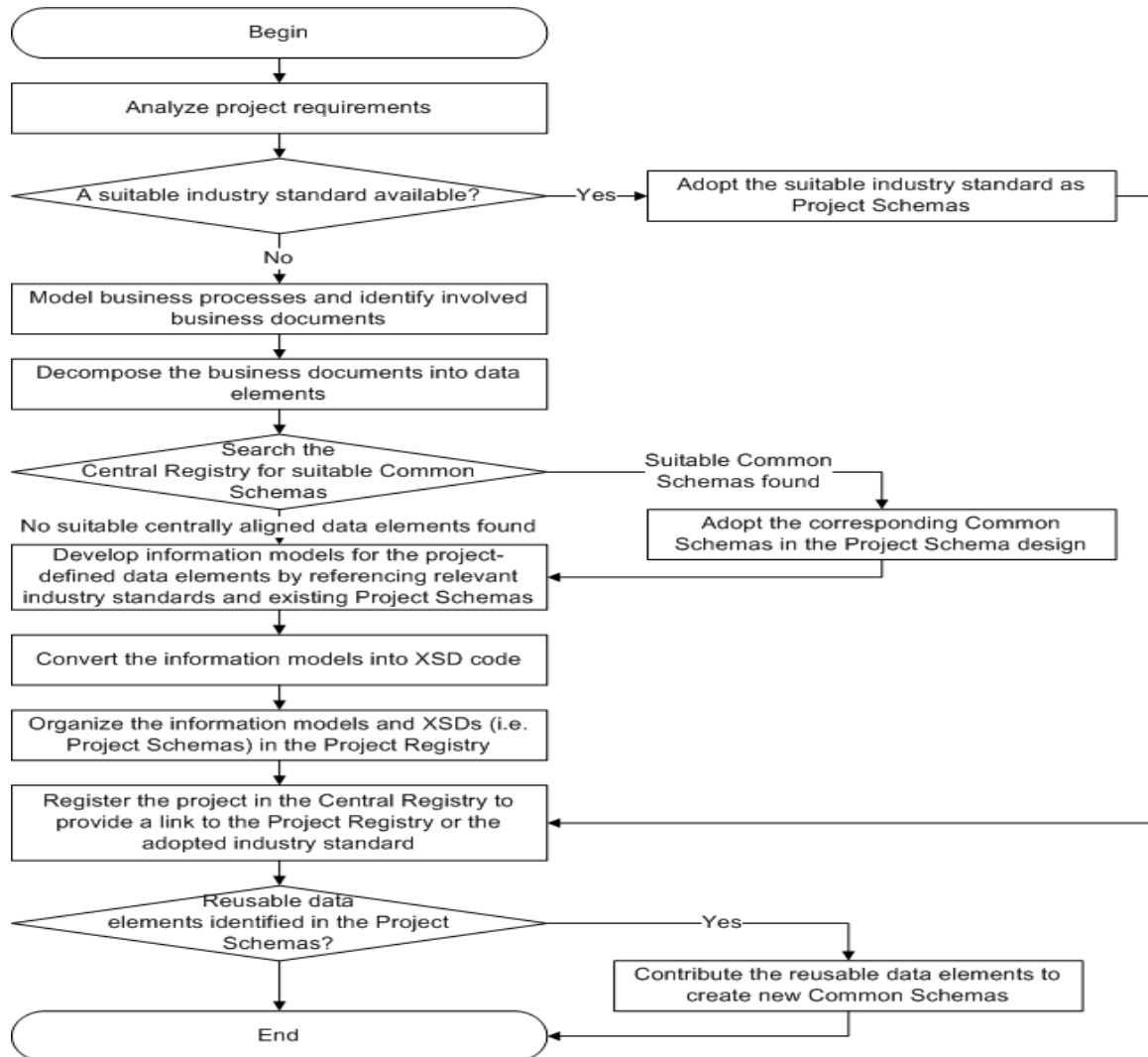
Figure 1: XML schema design process
