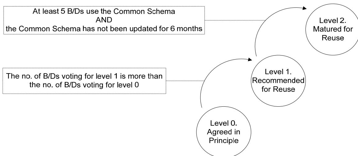
Figure 5: Promotion of the maturity level of a common schema
