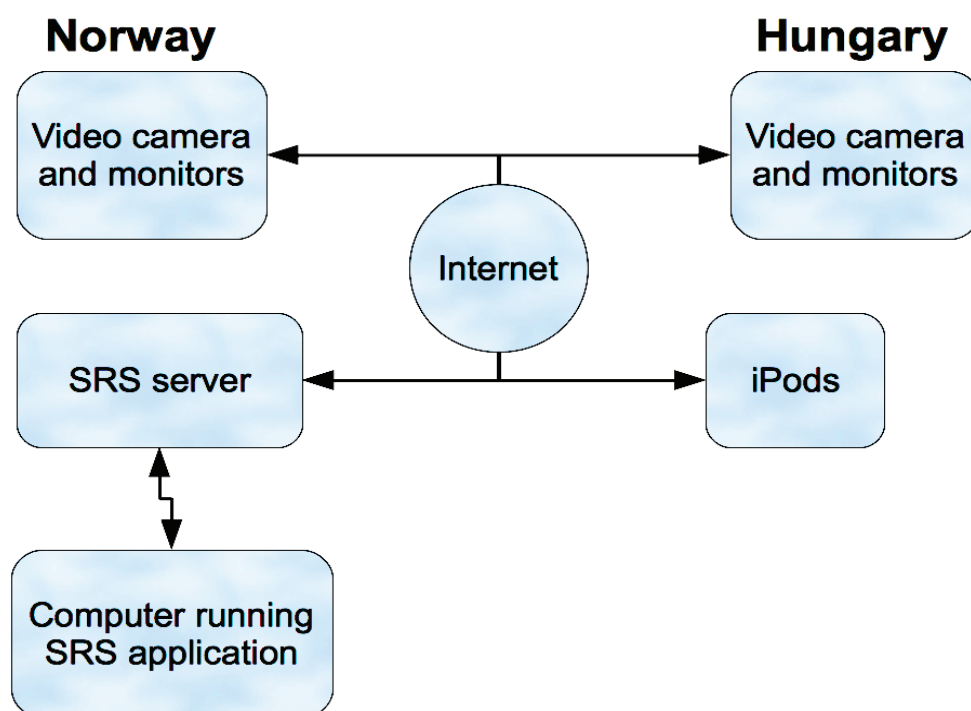
Figure 3: A schematic outline of the video and SRS IP based communication infrastructure during an instruction-training course from Trondheim, Norway, to Visonta, Hungary the teacher (in Norway) and participants communicate two-way by use of video conferencing. The teacher is running the SRS application on a digital blackboard and the participants can see the display on their monitors
