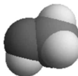
Figure 6: 3D Model of methanol (non-space filling and space filling) from the programme Wolfram|Alpha
