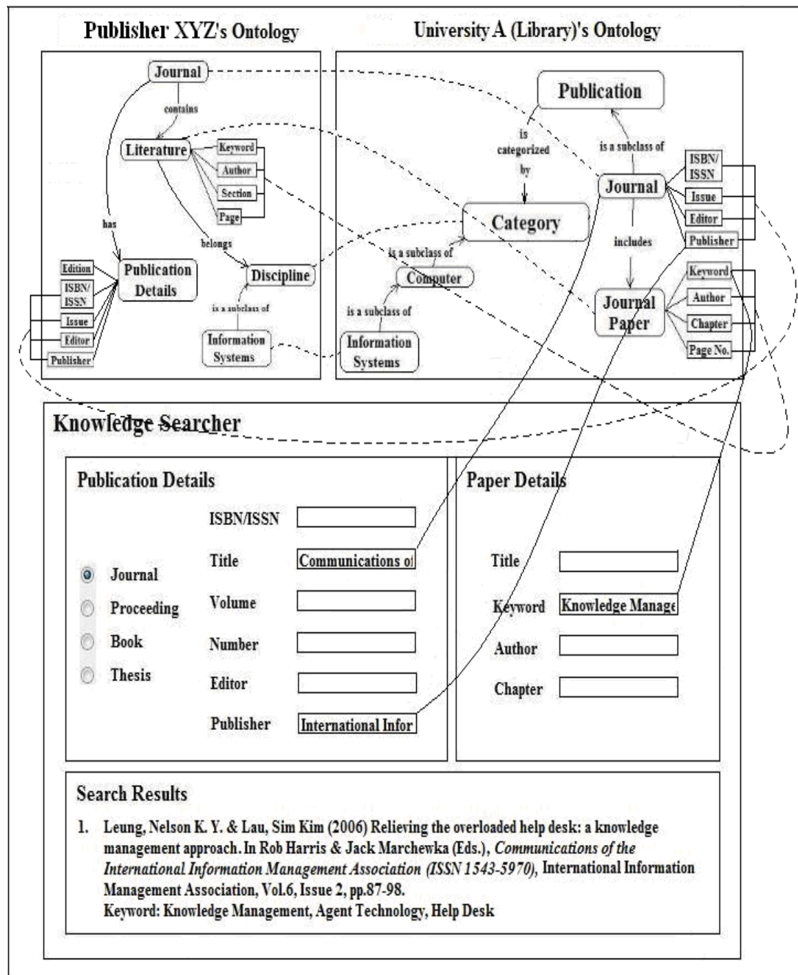
Figure 6: Inter-organizational knowledge retrieval and reusing process
